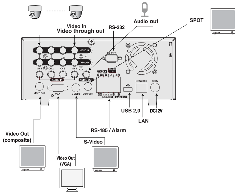
[SHR-2040]
