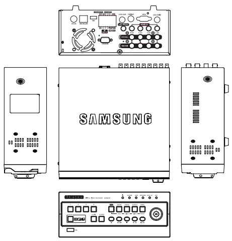
[SHR-2040]
