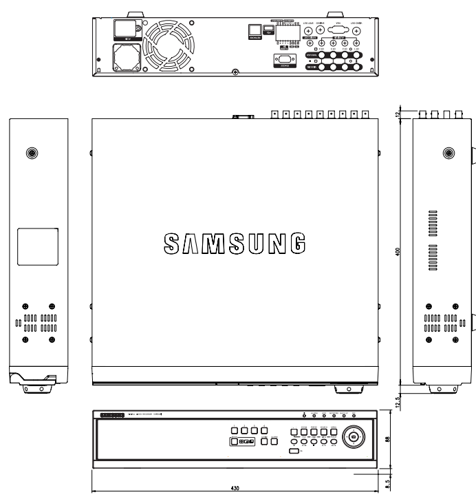
[SHR-2041]
