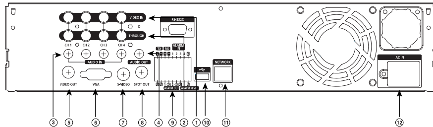
[SHR-2041/2042]
