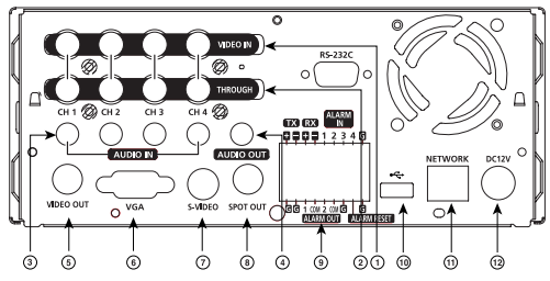
[SHR-2040]
