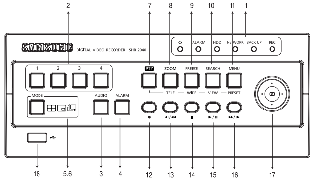
[SHR-2040]
